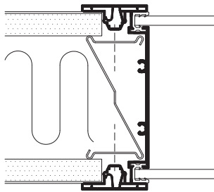
Gypsum board/glass joint horizontal section
