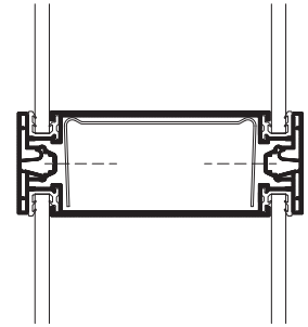
Glass joint vertical section
