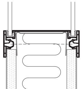
Gypsum board/glass joint vertical section
